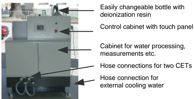
Fig. 4: Front view of CEU 120
