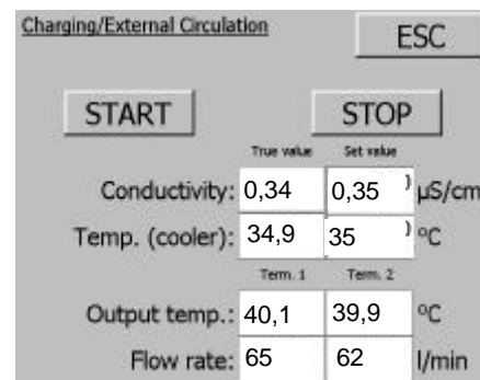
Fig. 6: Visualization of key parameters on the CEU touch screen during testing
