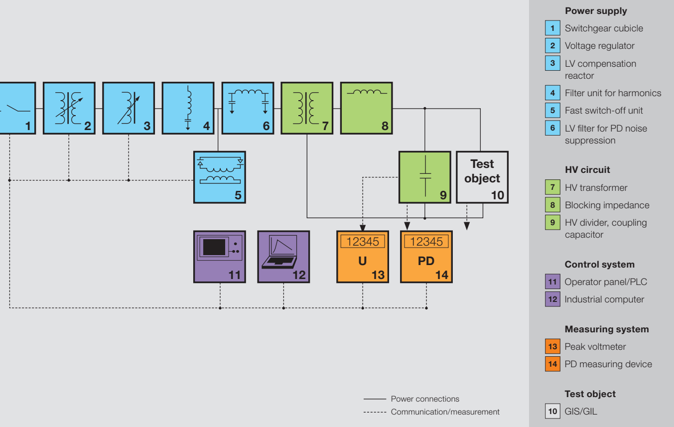
Fig. 4 Block diagram of AC testing of GIS with transformer based test systems
