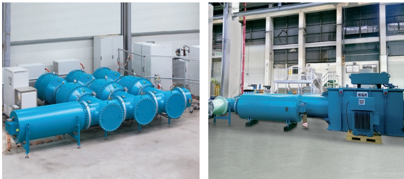
Fig. 10 AC test system WRVG 5.7/750 G (gas-insulated reactors, left side) and WRV 6/750 G (oil-insulated reactor, right side)
