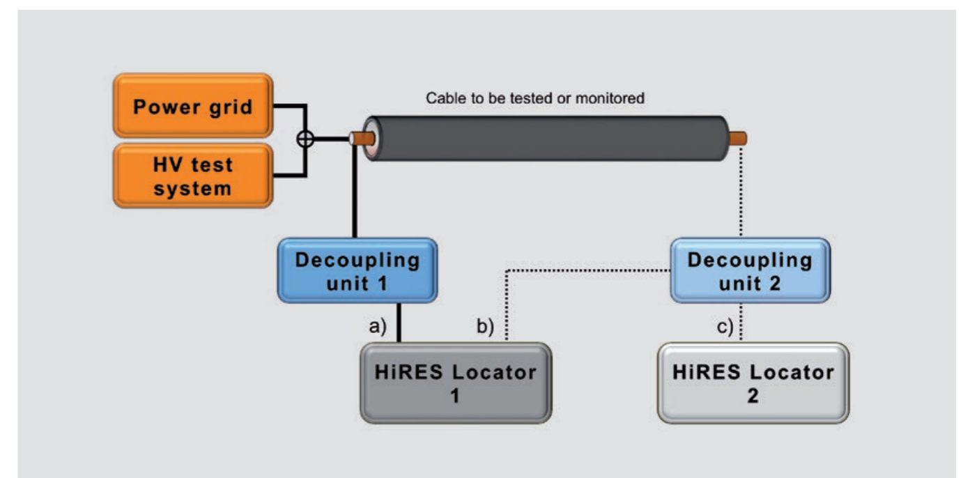
Fig. 5 Functional principle of the HiRES Locator (representation of one phase in a three-phase cable system; measurement optionally possible at both cable ends)
