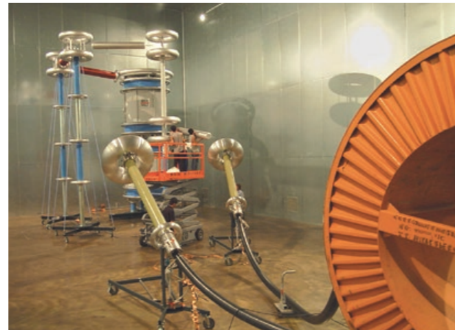
Fig. 2 Factory cable testing with HiRES Locator and AC resonant test system WRM
