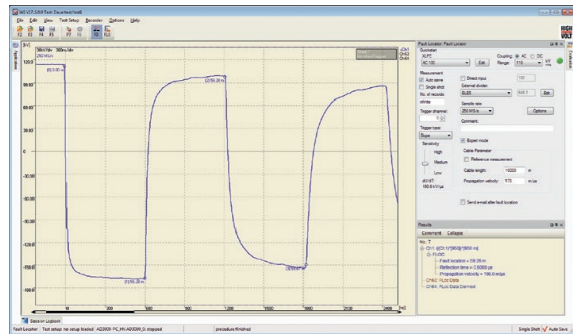
Fig. 6 Screenshot of the software for breakdown localization IAS LOC
