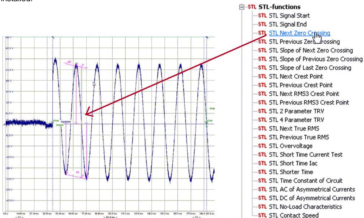
Figure 1: Function of HiRES Advanced STL software module
