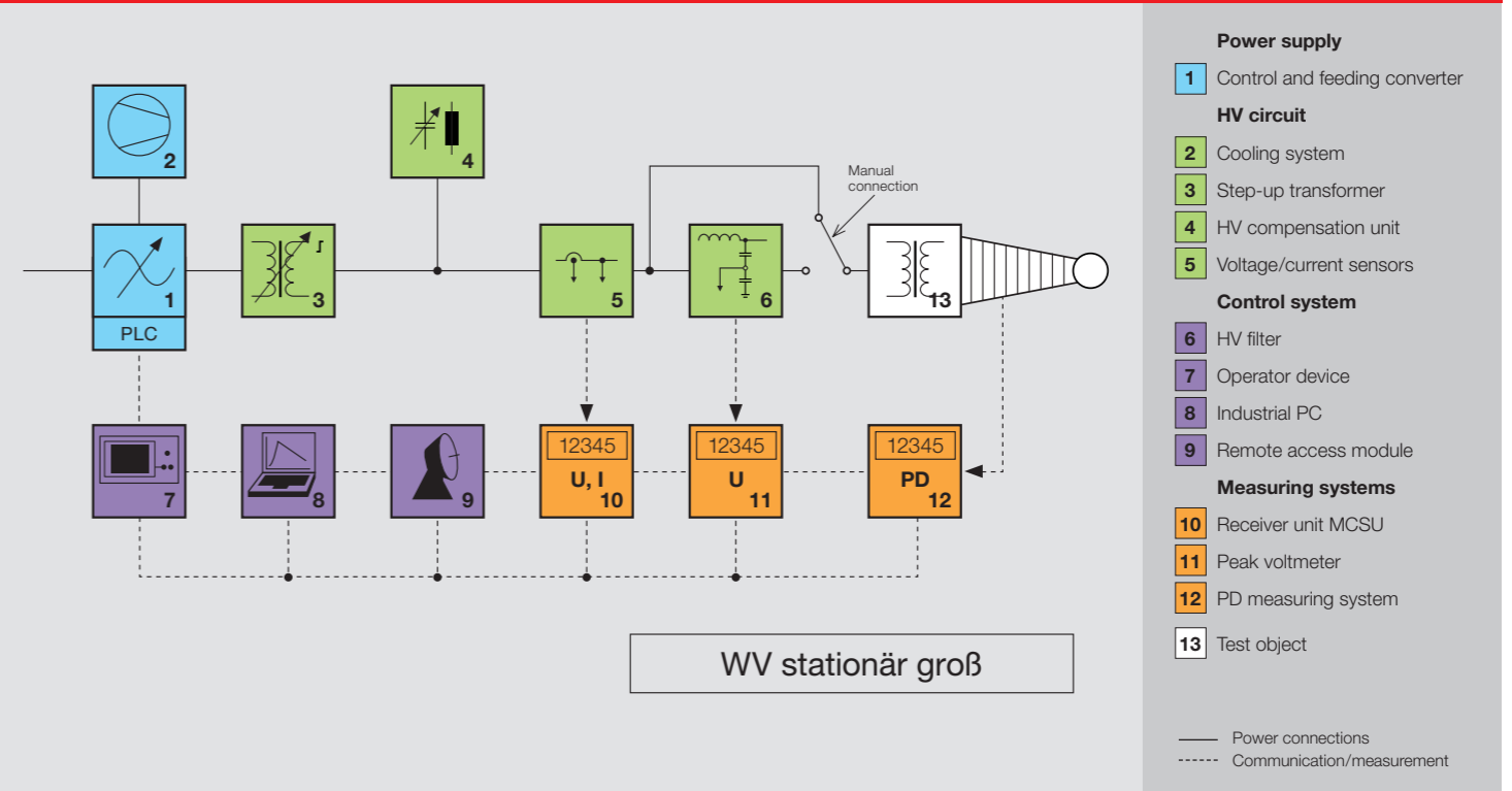
Fig. 2 Block diagram of transformer test system
